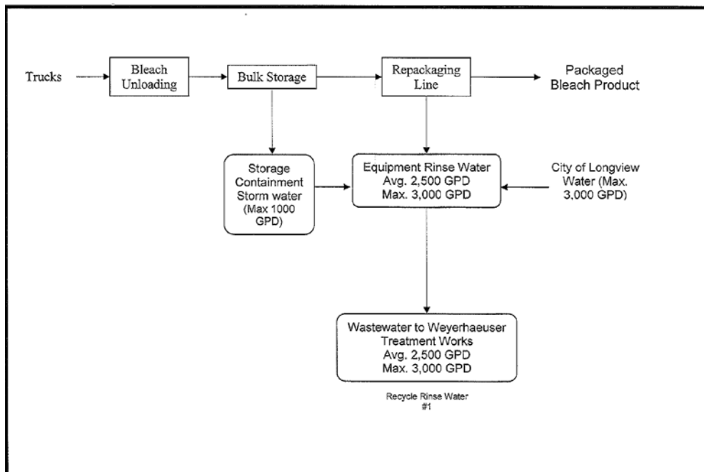
Figure 2 Site Schematic
