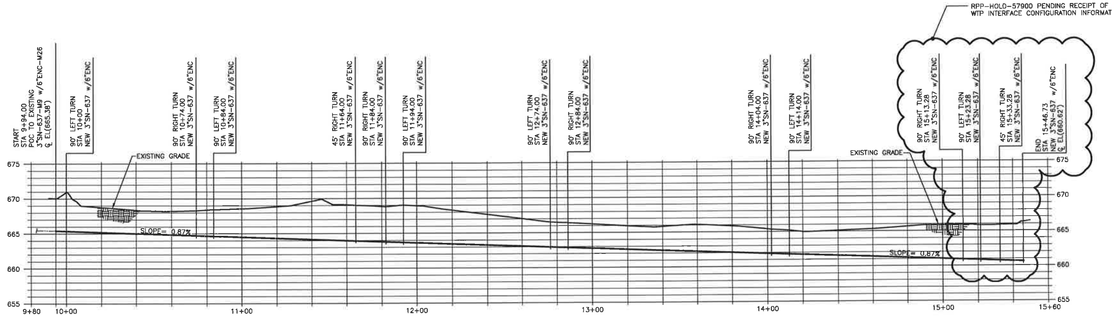
PROFILE NEW 3"AP06A-WT-WTL-SN-637 SCALE - HORIZONTAL: 1"=20' VERTICAL: 1"=5'
